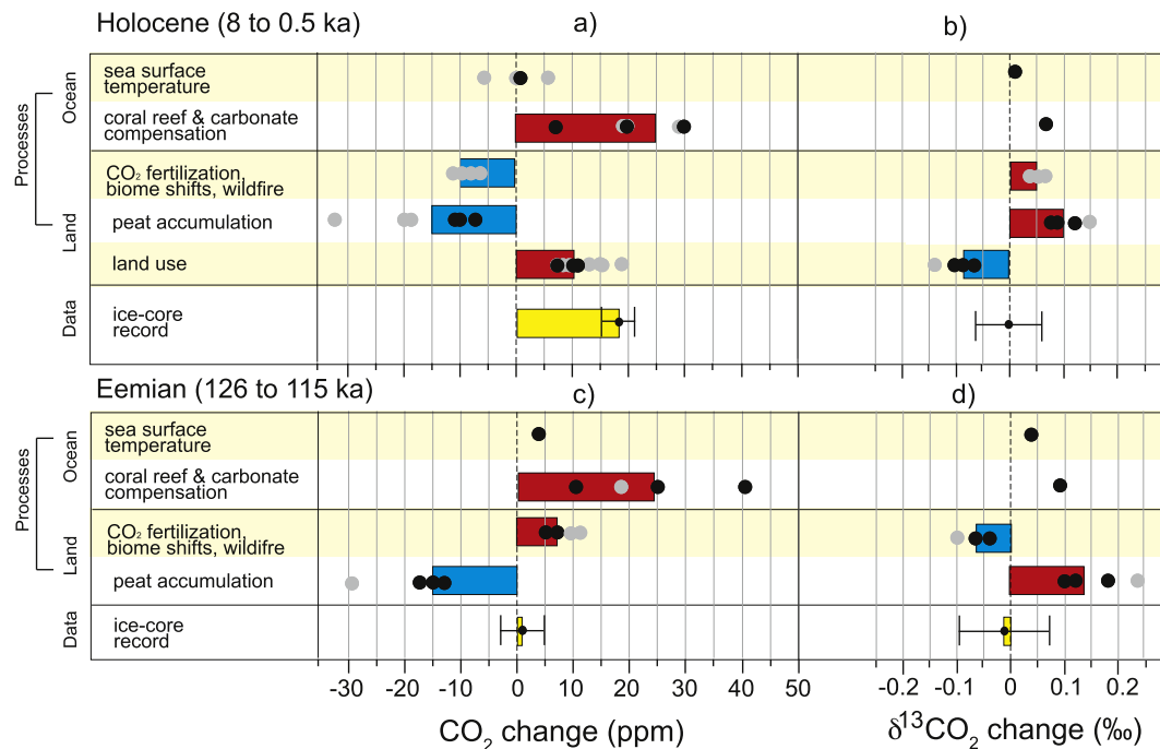
Fig. 8. Relative contributions of different processes to changes in atmospheric \text{CO}_2 concentration, ppm (a, c) and \delta^{13}\text{C}_{\text{CO}_2} ‰ (b, d) during the Holocene (a, b) and the Eemian (c, d). Gray dots are for previous studies incl. (Kleinen et al., 2015) while black dots and uncertainty ranges are for the given study. After Fig. 6.5 in Ciais et al. (2013) modified from Kohfeld and Ridgwell (2009).
